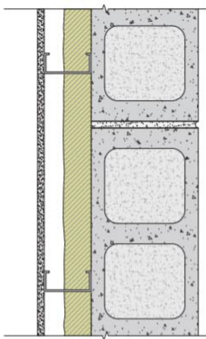
Option 1 R-12 Cavity Insulation
