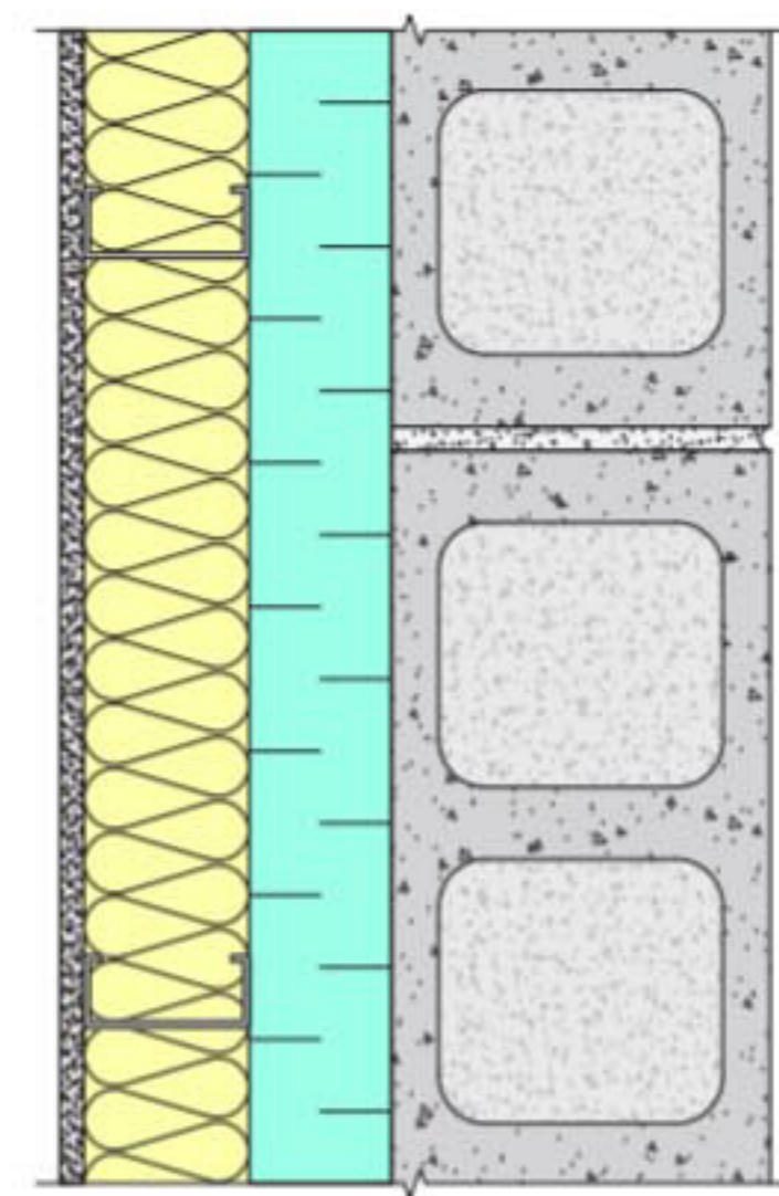
Option 8 R-15 Cavity Insulation R-15 Continuous Insulation
