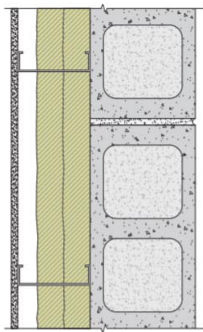
Option 6 R-24 Cavity Insulation
