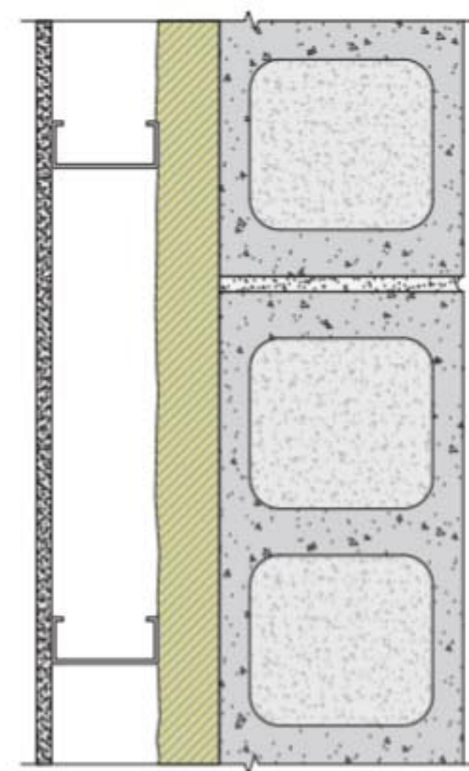
Option 4 R-12 Continuous Insulation
