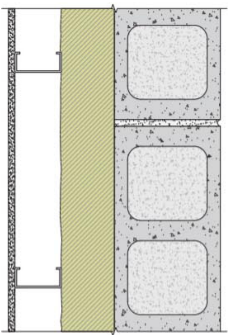
Option 5 R-24 Continuous Insulation
