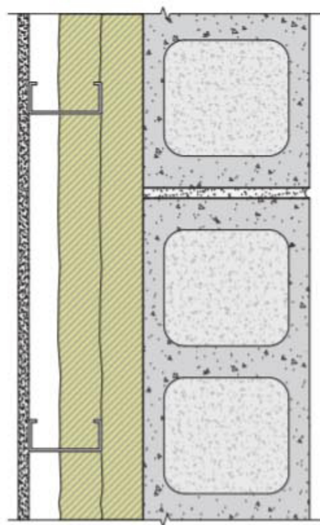
Option 2 R-12 Cavity Insulation with R-12 Continuous Insulation
