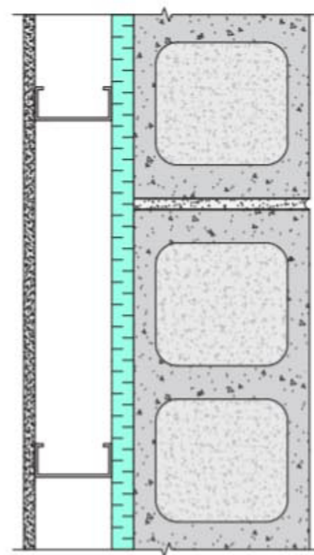
Option 3 R-5 Continuous Insulation
