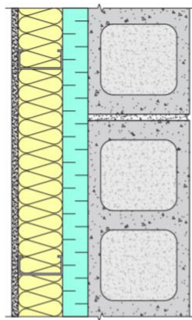
Option 7 R-15 Cavity Insulation R-10 Continuous Insulation
