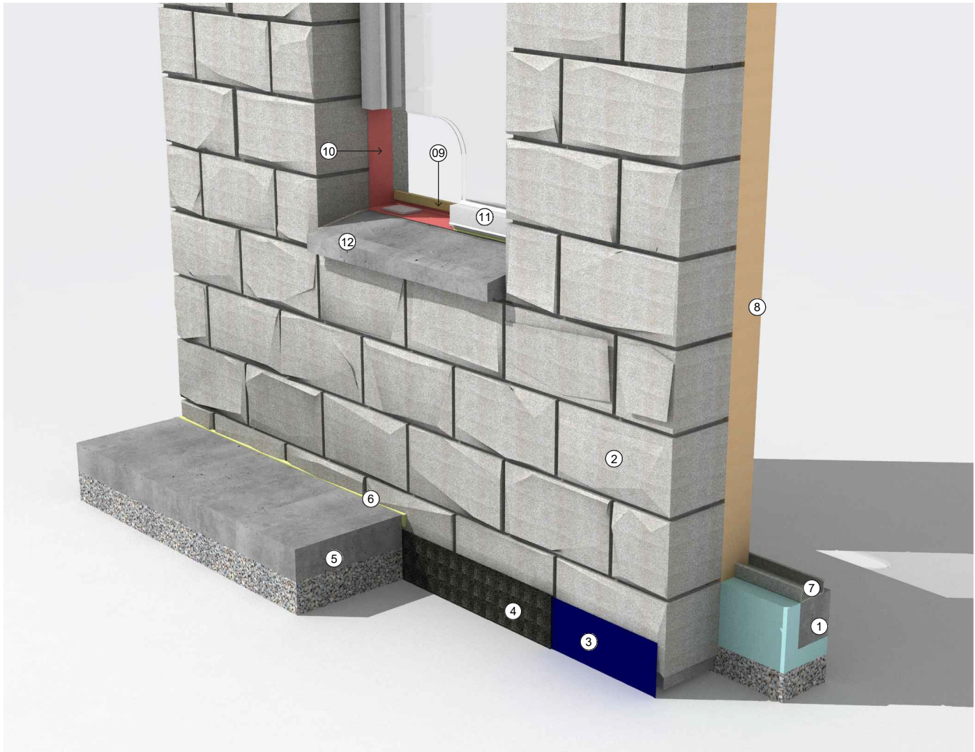
Detail 7-7 Single-Wythe CMU Wall: Base-of-Wall 3D Detail
