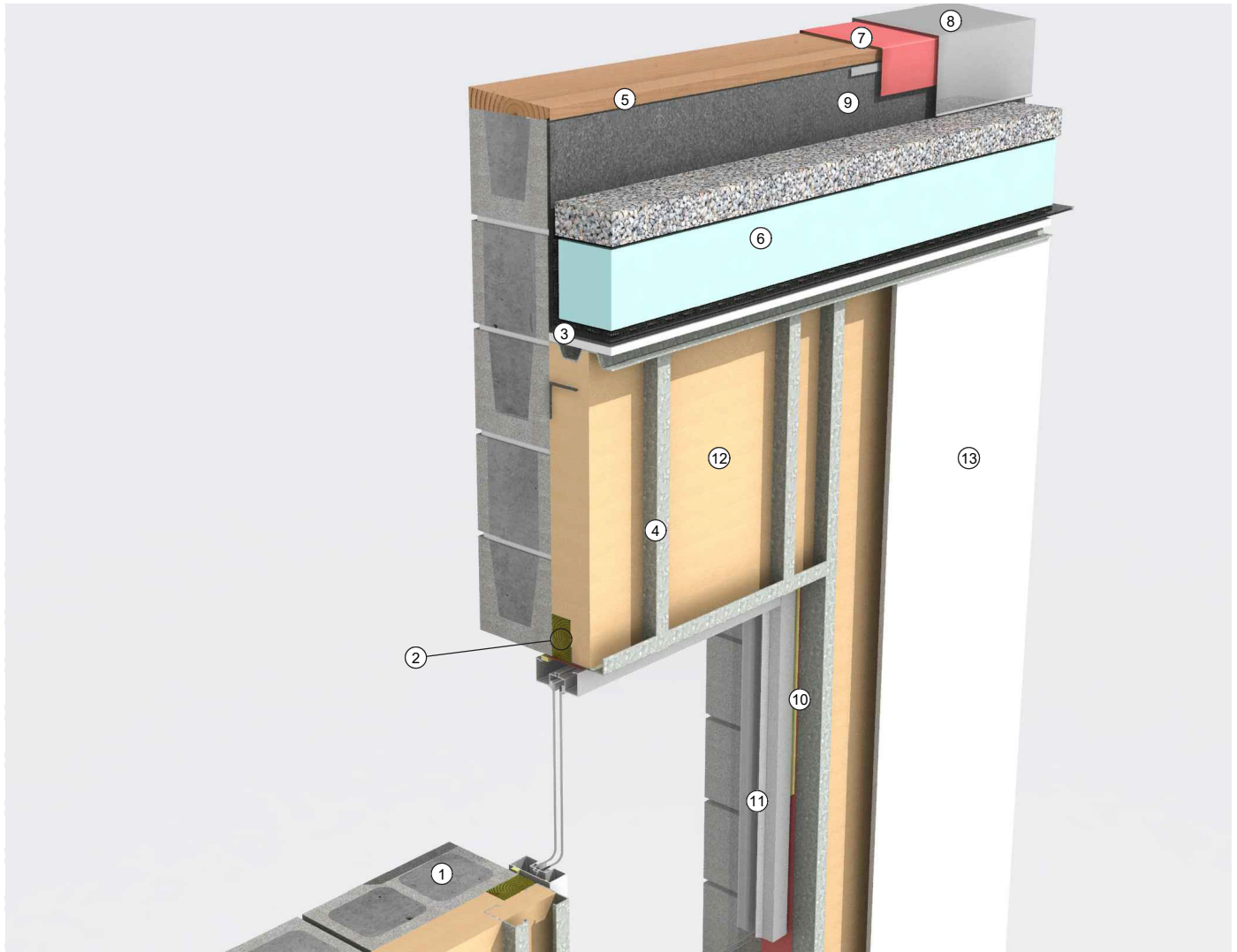
Detail 7-6 Single-Wythe CMU Wall: Roof Parapet 3D Detail
